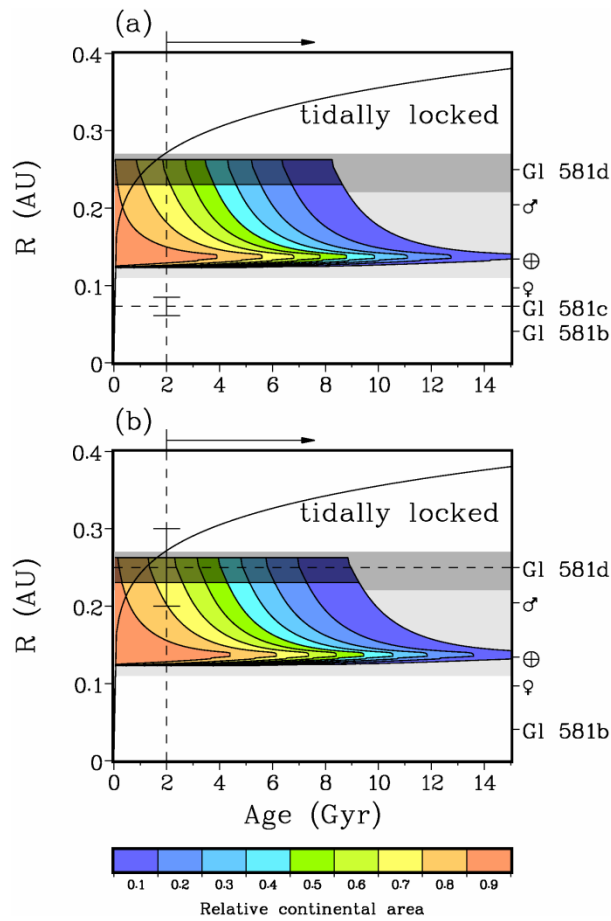
Figure 2: The pHZ of Gl 581 for super-Earth Gl 581c (a) and Gl 581d (b) with a relative continental area varied from 0.1 to 0.9 and a stellar luminosity of 0.013 L_{\odot} as a function of planetary age. The light colours correspond to a maximum CO 2 pressure of 5 bar, whereas the dark colours correspond to 10 bar. For comparison, the positions of Venus, Earth and Mars are shown scaled to the luminosity of Gl 581. The light and dark grey shaded areas denote different approximations for the so-called stellar HZ. The vertical bar at 2 Gyr denotes the range of distances due to the (possibly) eccentric orbit. The area below the solid black curve is affected by tidal locking [3].
