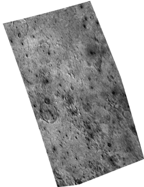
Fig. 4. An image of slope of polarization phase curve at the inversion angle h for the region shown in Fig. 1.
