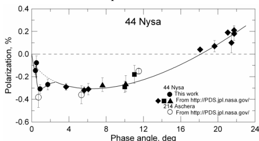
Fig. 1. The phase-angle dependence of polarization for asteroid 44 Nysa. The averaged in the BVRI filters values of polarization for asteroid 214 Aschera are also shown (data are taken from [6]).
